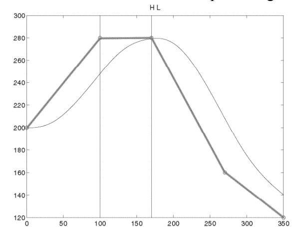
b. Less undershoot in HL with spread target
